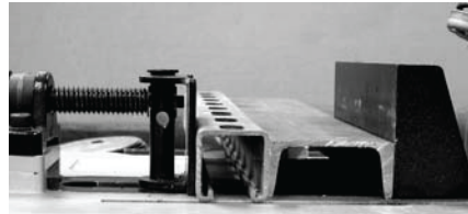
Channels & UNISTRUT™ (use block spacer)
