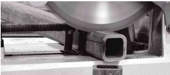
Carbide-Tipped Blades make Virtually Spark-Free Cuts
